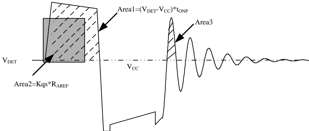
Figure 3. AREF Function
