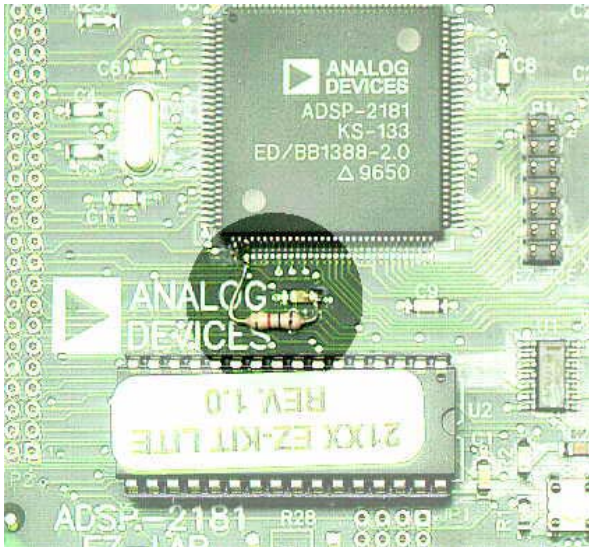
Figure 1: BMODE pin change
