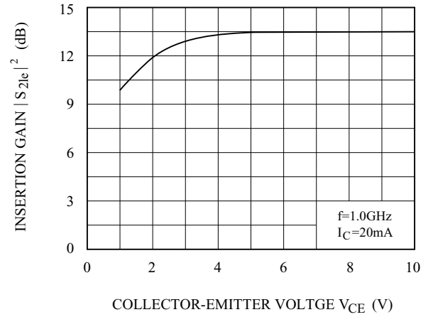
|S_{2le}|^2 - V_{CE}
