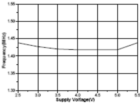
Figure 6. Frequency vs. Supply Voltage
