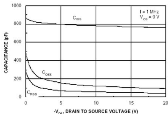
Figure 8. Capacitance Characteristic
