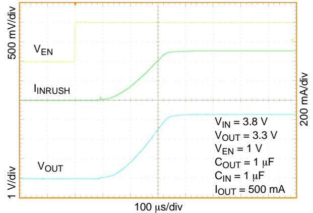
Figure 43. Enable Turn-on Response, C_{OUT} = 1\text{ }\mu\text{F} , I_{OUT} = 500\text{ mA}
