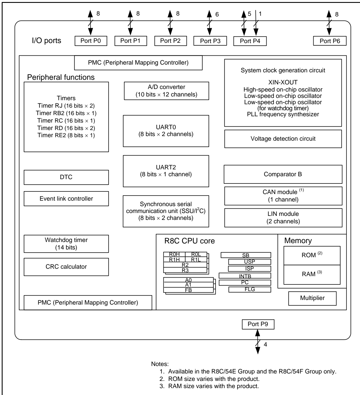
Figure 1.5 Block Diagram
