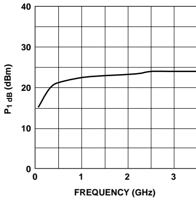
Figure 4. Output Power vs. Frequency. V_{\text{Control}} = -7 \text{ V.}
