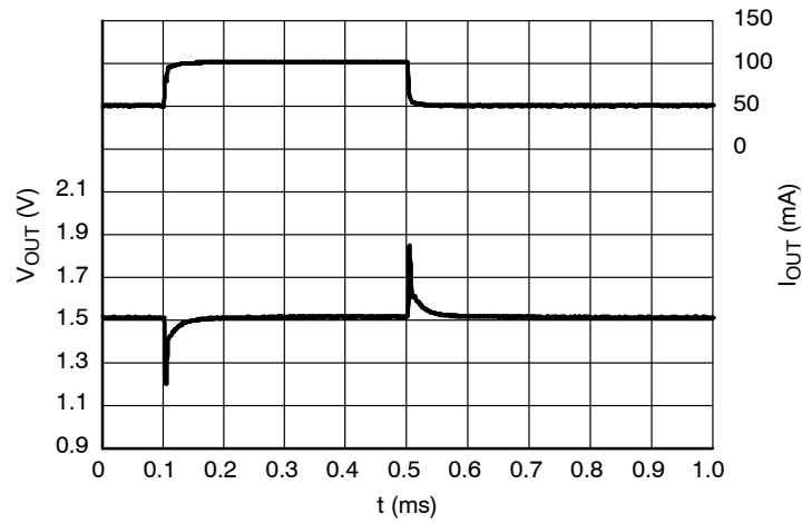
Figure 26. Load Transients, 1.5 V Version, I_{OUT} = 50 - 100 \text{ mA} , t_R = t_F = 0.5 \mu s , V_{IN} = 2.5 \text{ V}
