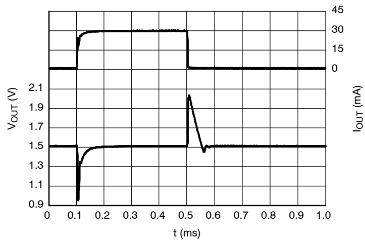
Figure 32. Load Transients, 1.5 V Version, I_{OUT} = 1 - 30 mA, t_R = t_F = 0.5 \mu s, V_{IN} = 2.5 V
