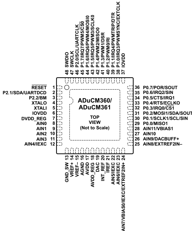
Figure 8. Pin Configuration
