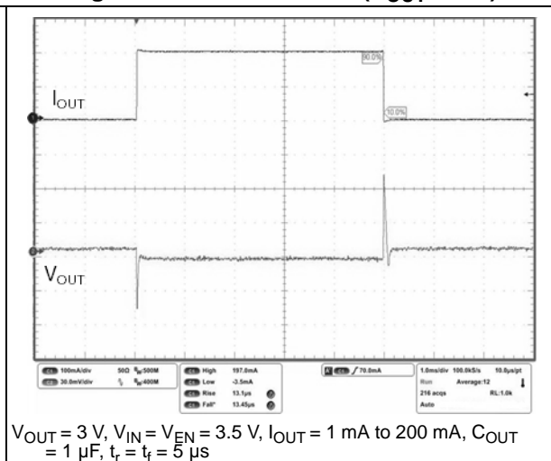
Figure 29. Load transient ( V_{OUT} = 3\text{ V} )
