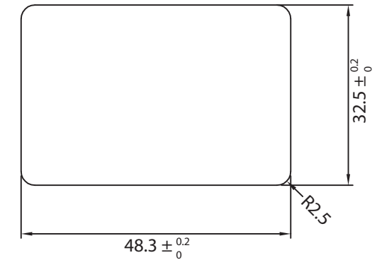
PANEL CUTOUT
