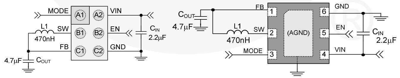
Figure 1. Typical Applications
