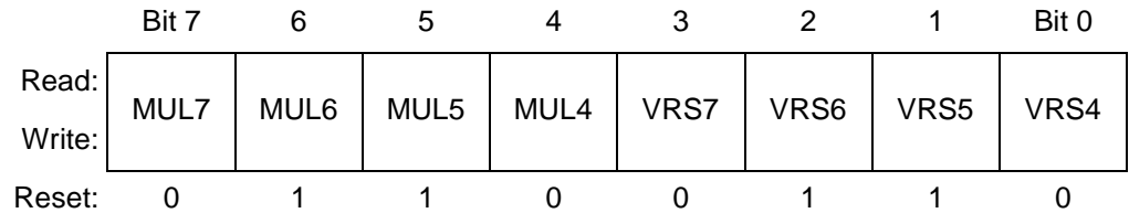
Figure 8-7. PLL Programming Register (PPG)
