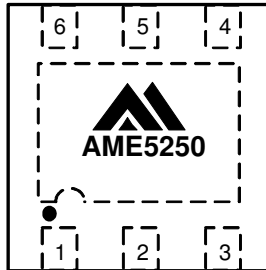
DFN-6D (2mmx2mmx0.75mm) Top View
