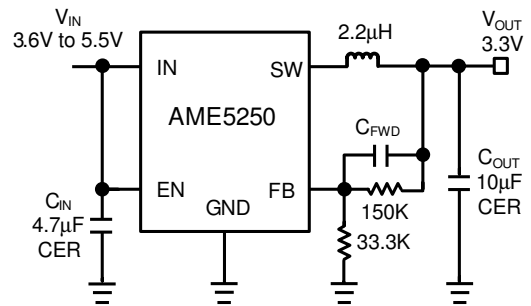
Figure 9. 3.3V Step-Down Regulator C_{FWD} : 22pF~220pF
