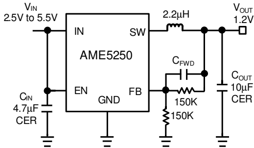
Figure 5. 1.2V Step-Down Regulator C_{FWD} : 22pF~220pF
