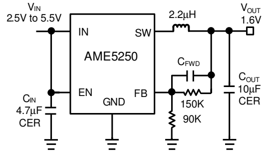
Figure 8. 1.6V Step-Down Regulator C_{FWD} : 22pF~220pF
