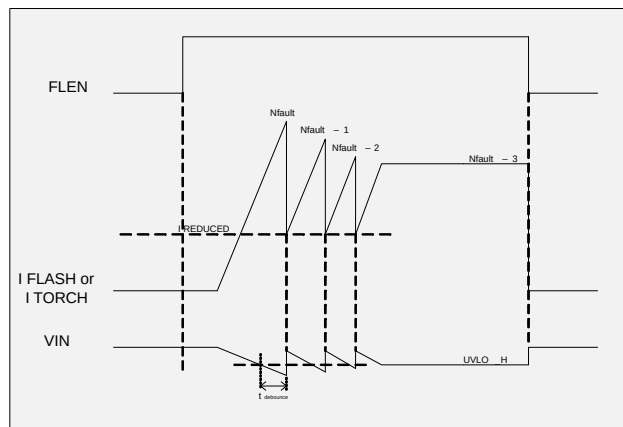
Figure 25. Battery Voltage Adaptive Mode Behavior
