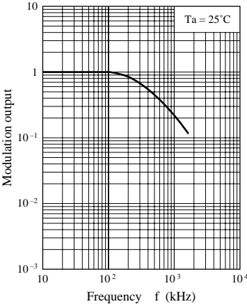
Frequency characteristics
