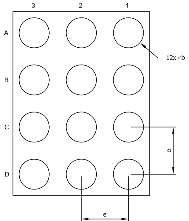
Bottom View
