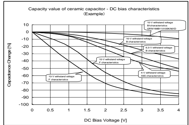
Figure 14. Capacity-bias characteristics
