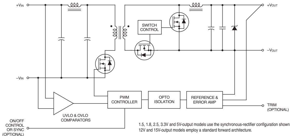
Figure 1. Simplified Schematic
