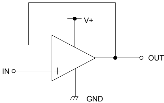
Figure 85. Voltage Follower
