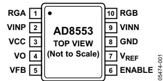
Figure 1. 10-Lead MSOP
