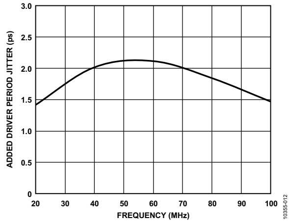
Figure 12. Driver Jitter (Period) vs. Frequency ( V_{CC} = 3.3 V , T_A = 25^\circ C , Clock Input)
