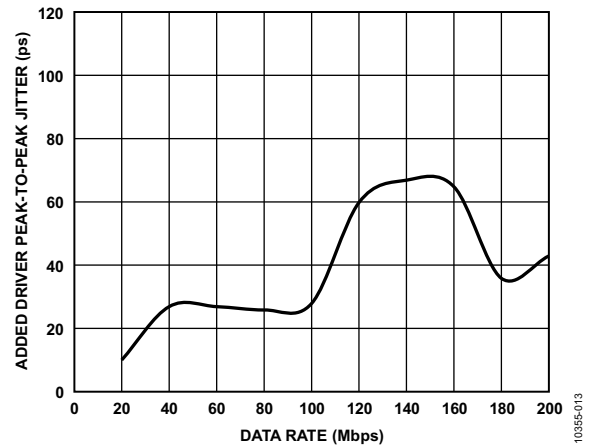
Figure 13. Driver Jitter (Peak-to-Peak) vs. Data Rate ( V_{CC} = 3.3 V , T_A = 25^\circ C , PRBS 2^{15} - 1 Input)
