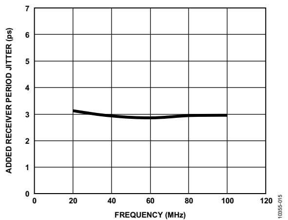
Figure 15. Receiver Jitter (Period) vs. Frequency ( V_{CC} = 3.3 V , T_A = 25^\circ C , V_{ID} = 400 mV )
