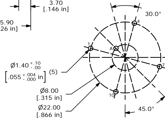
P.C. MOUNTING
