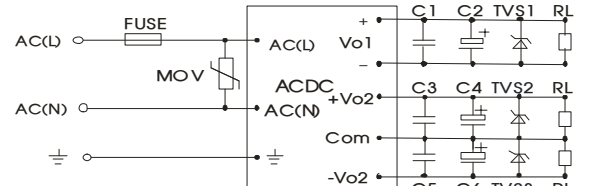
Fig. 4: LH15-10Cxx (Triple Output) series typical application circuit
