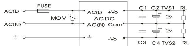
Fig. 2: LH15-10Axx (Dual Output) series typical application circuit
