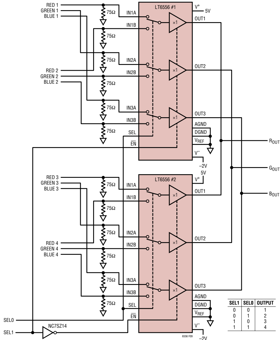
Figure 9. 4:1 RGB Multiplexer
