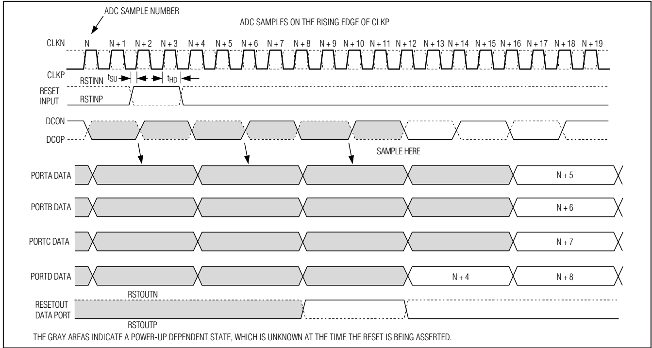
Figure 16. Reset Output Timing in Demultiplexed SDR Mode
