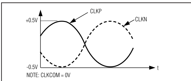
Figure 13b. Differential Clock Input—Sine-Wave Drive
