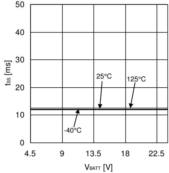
Figure 24. Soft-start Time
