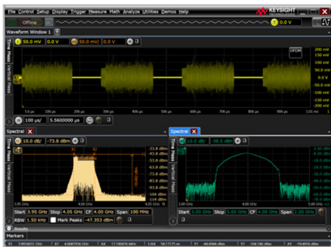
Use Infiniium capture and analysis of radar bursts, as shown in this OFDM example.
