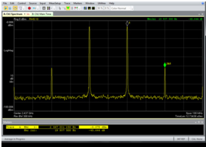
Using data acquired from S-Series, VSA shows an excellent TOI value of 21.5 dB.
