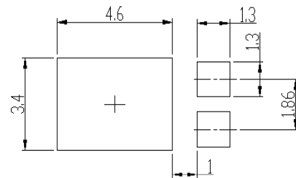
Soldering footprint
