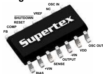
14-Lead SOIC (Narrow Body)
