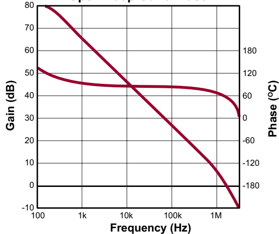
Fig. 5 Error Amplifier Open Loop Gain/Phase
