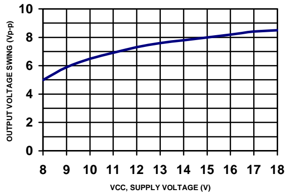
Figure 6. Output Voltage Swing
