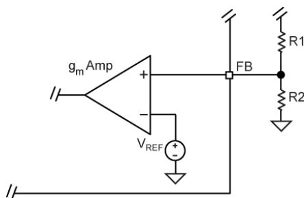
Figure 7. Voltage-Divider Configuration
