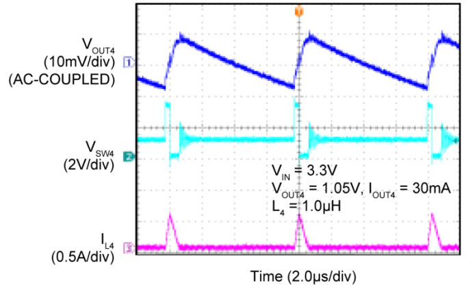
Buck 4 PFM Switching Waveforms
