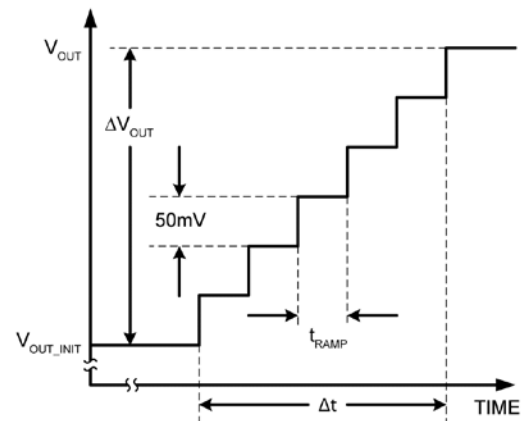
Figure 3. Buck DVC Control Ramp
