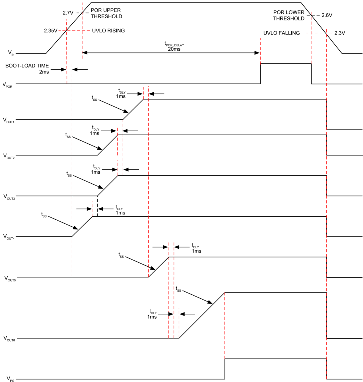
Figure 19. MIC7401 Power-Up/Down
