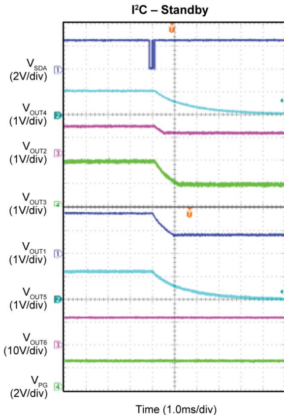
Figure 12. I 2 C Stand-By Mode
