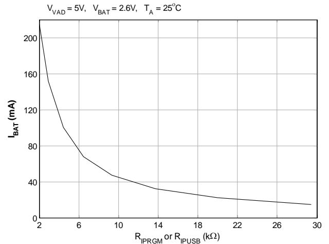
I_{PQ\_AD} vs. R_{IPRGM} , or I_{PQ\_USB} vs. R_{IPUSB}
