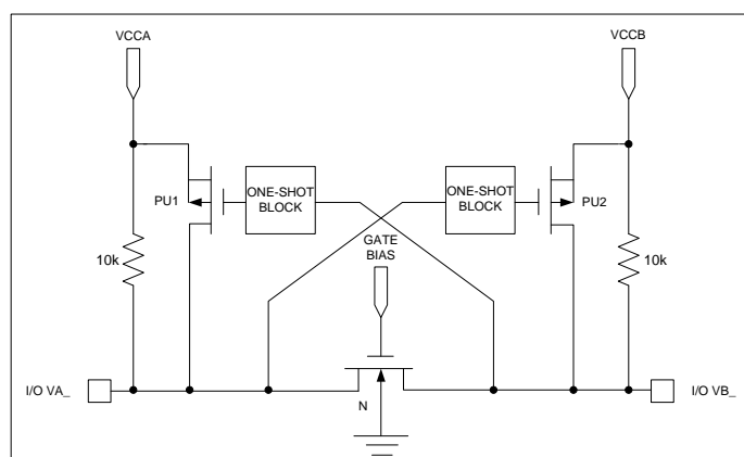
Figure 1 Block Diagram of UM3202Q/3202A/3202H/3202V I/O Cell
