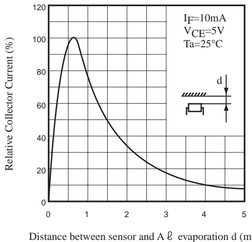
Relative Collector Current vs. Distance
