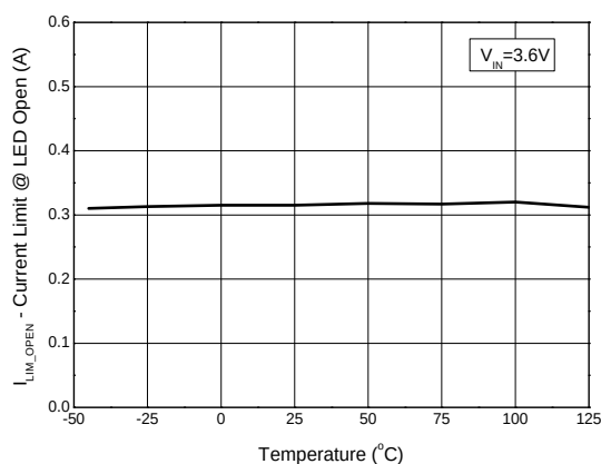
Current Limit @LED Open vs. Temperature
