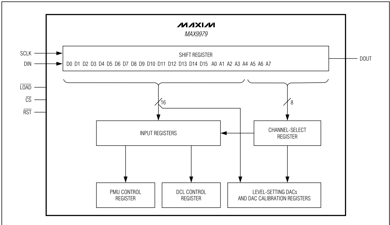
Figure 8. Serial-Interface Block Diagram
