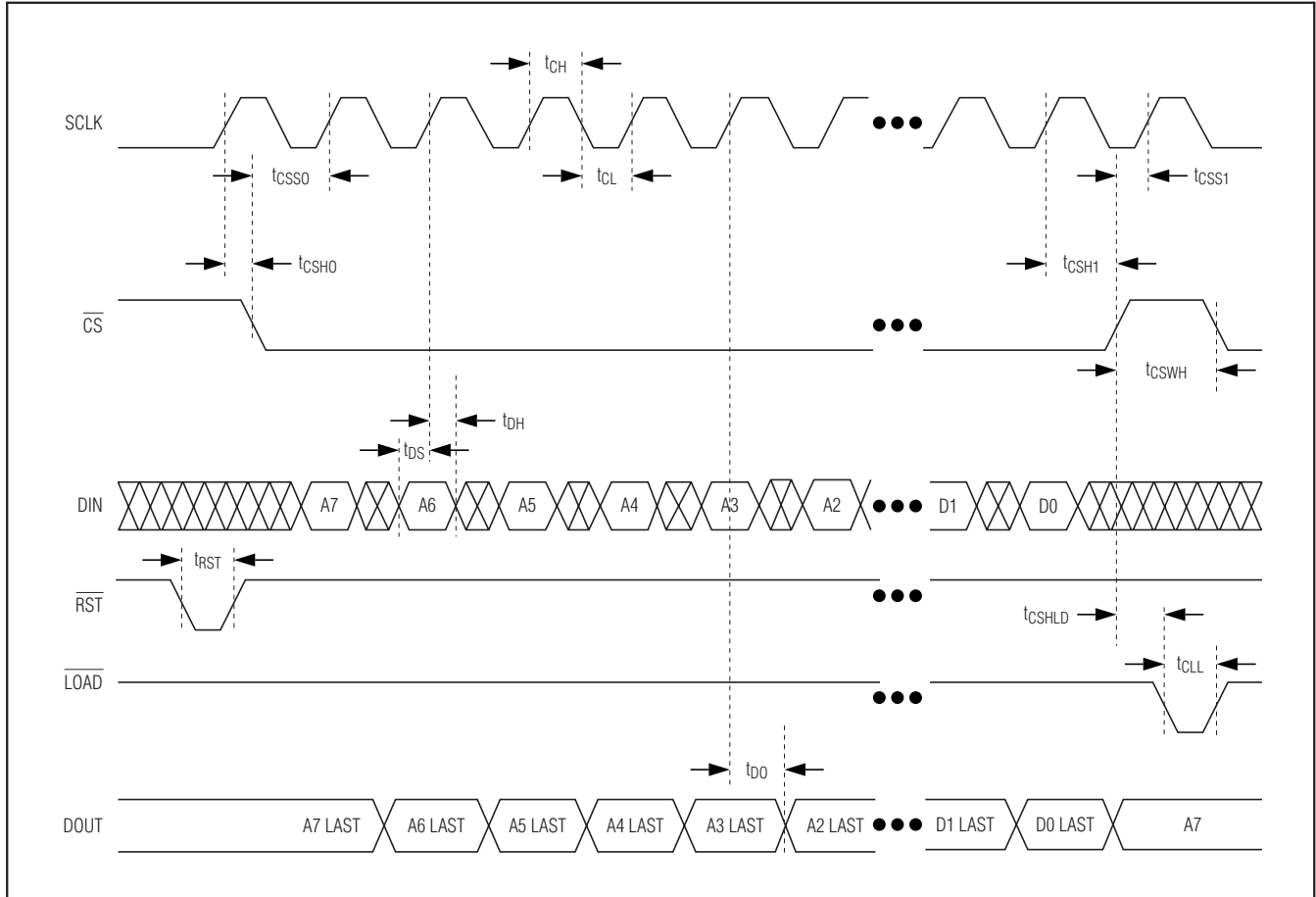
Figure 9. Serial-Interface Timing
