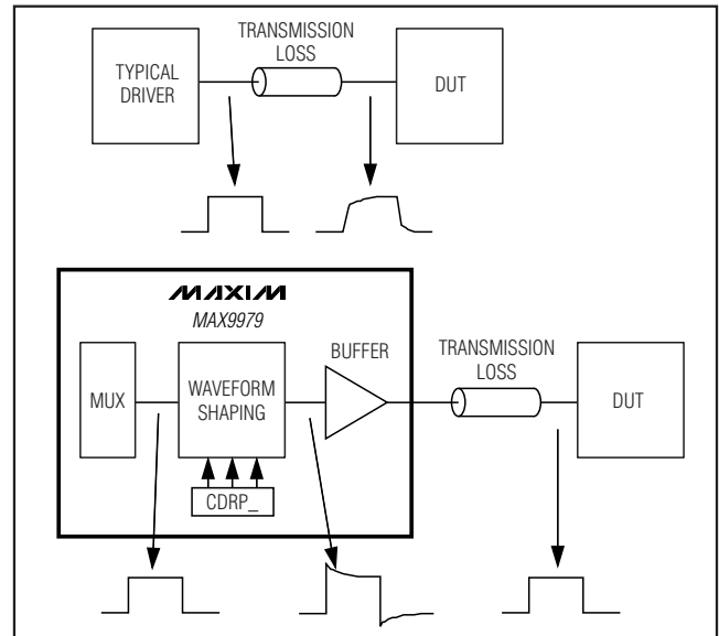
Figure 2. Cable-Droop Compensation
