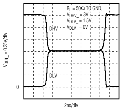
DRIVER-TO-TERM TRANSITION
