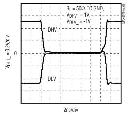
DRIVER TO HIGH-IMPEDANCE TRANSITION
