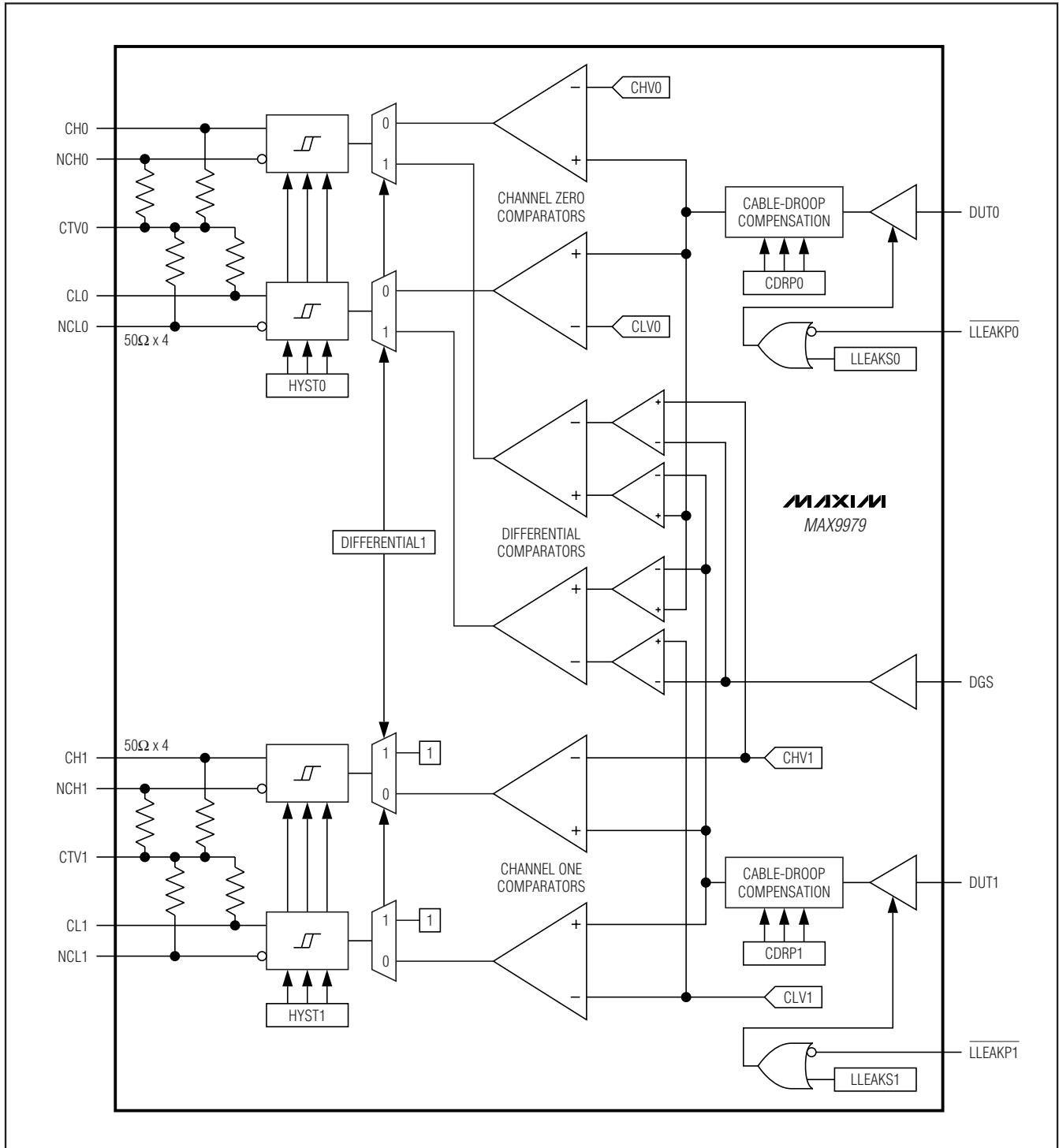
Figure 4. High-Speed Comparators Block Diagram
