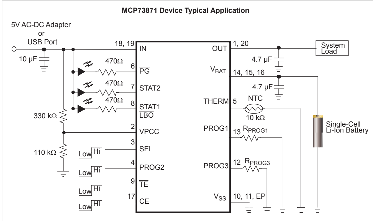
FIGURE 6-1: MCP73871 Typical Stand-Alone Application Circuit with VPCV.
