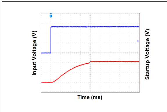
FIGURE 2-25: Startup Delay.
