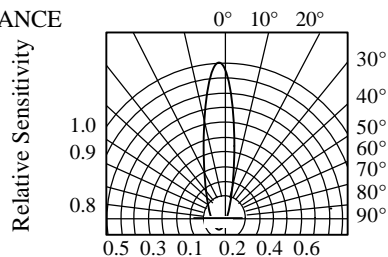
FIG.5 SENSITIVITY DIAGRAM
