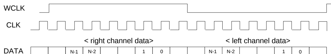
Figure 35: I2S format
