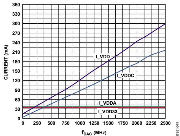
Figure 74. Current Consumption vs. f DAC @ 25°C
