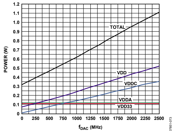
Figure 73. Power Consumption vs. f DAC @ 25°C
