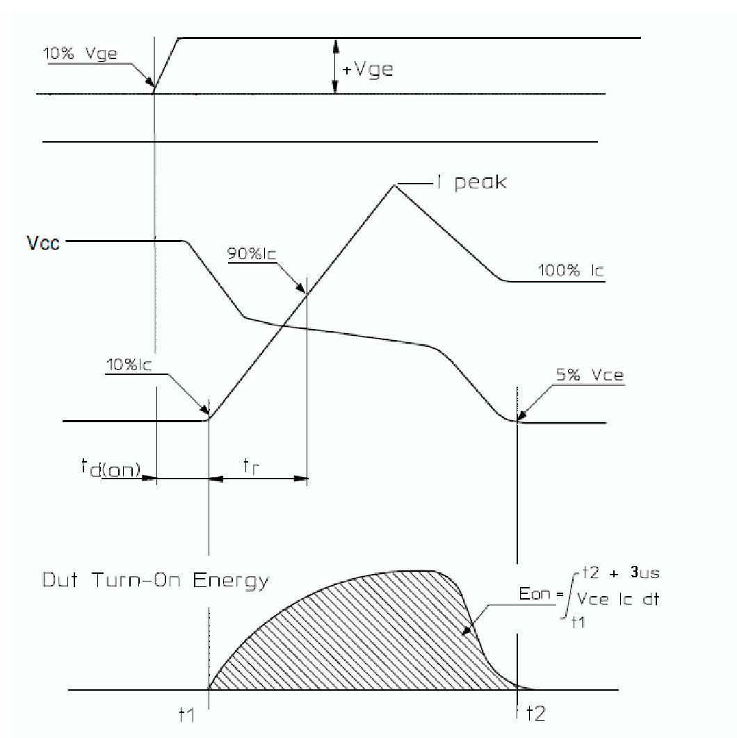
Figure 21. Definition of Turn On Waveform
