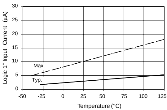
Figure 19A. Logic "1" Input Current vs. Temperature
