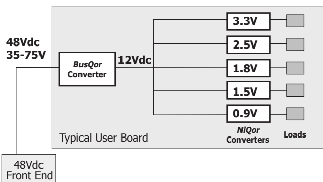
Figure A: Example of Intermediate Bus Architecture using BusQor bus converter and NiQor non-isolated converters
