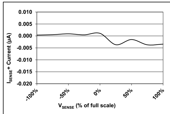
FIGURE 2-11: I SENSE- Pin Leakage Current, T A = -40°C to +85°C.
