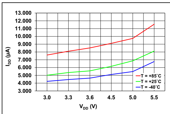
FIGURE 2-9: I DD vs. V DD , Standby Mode (PAC1720).
