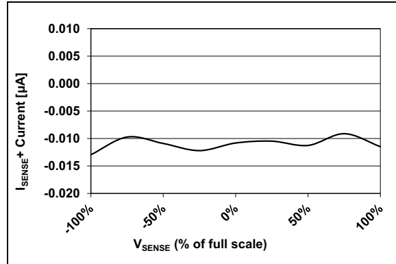
FIGURE 2-10: I SENSE+ Pin Leakage Current, T A = -40°C to +85°C.
