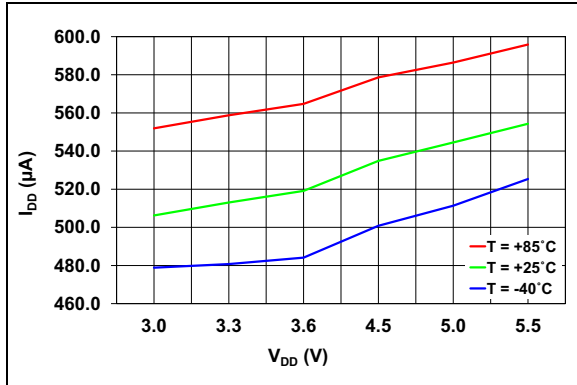
FIGURE 2-7: I DD vs. V DD , Continuous Conversions (PAC1720).
