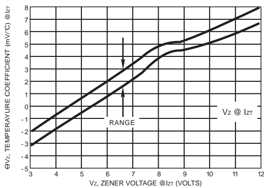
FIG.4- UNIT TO 12 VOLTS
