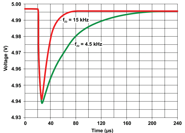
Figure 23: Transient Recovery Comparison for f_{Z2} at 4.5 kHz/63° and 15 kHz/51°.
