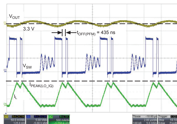
Figure 5: Low-IQ PFM Mode Operation at V_{IN} = 12\text{ V} , V_{OUT} = 3.3\text{ V} , and I_{OUT} = 330\text{ mA} . SW turns on only twice every 5 \mu\text{s} to regulate V_{OUT}
