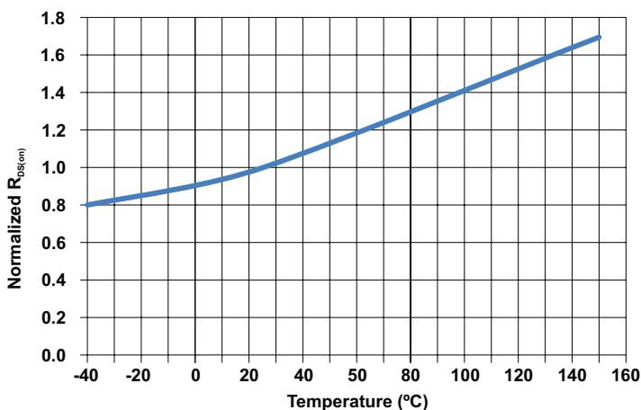
Figure 3: Typical MOSFET R_{\text{DS(on)}} versus Temperature
