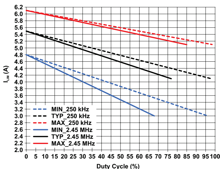
Figure 11: Pulse-by-Pulse Current Limit versus Duty Cycle
