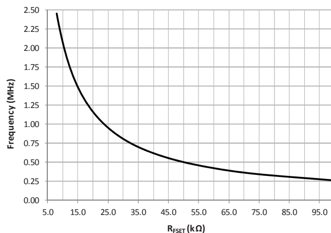
Figure 17: PWM Switching Frequency versus R_{FB1}
