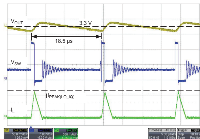
Figure 4: Low-IQ PFM Mode Operation at V_{IN} = 12\text{ V} , V_{OUT} = 3.3\text{ V} , and I_{OUT} = 66\text{ mA} . SW turns on only once every 18.5 \mu\text{s} to regulate V_{OUT}
