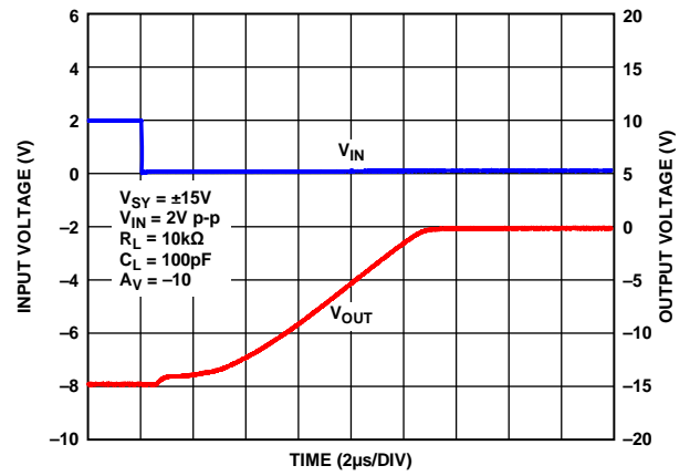
Figure 57. Negative Overload Recovery, V_{SY} = \pm 15\text{ V}
