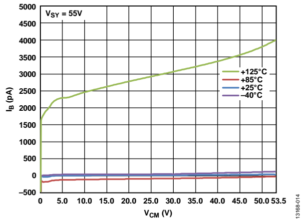
Figure 16. Input Bias Current ( I_B ) vs. Common-Mode Voltage ( V_{CM} ), V_{SY} = 55V
