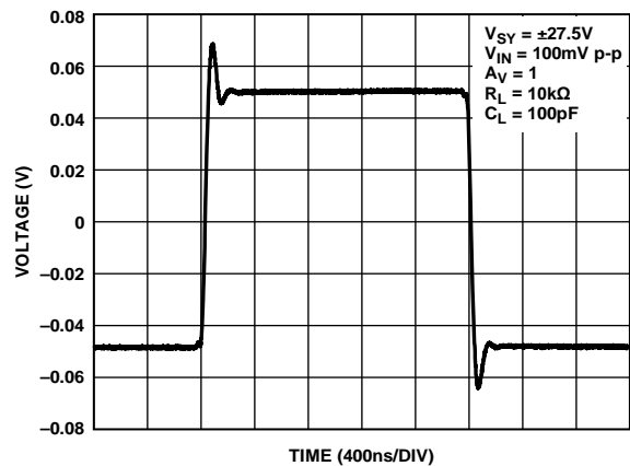
Figure 40. Small Signal Transient Response, V_{SY} = \pm 27.5 V
