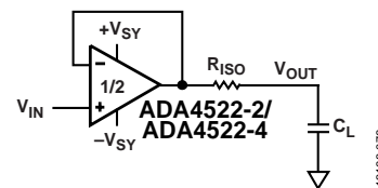
Figure 78. Stability Compensation with Isolating Resistor, R ISO
